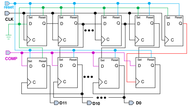
Fig. 5. Schematic of the SAR logic in digital DCOC
