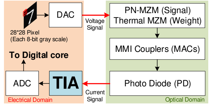
Fig. 1. The prototype of the PNN system
