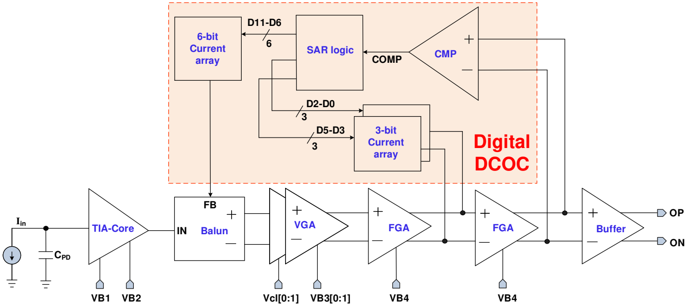
Fig. 2. System architecture of the proposed TIA
